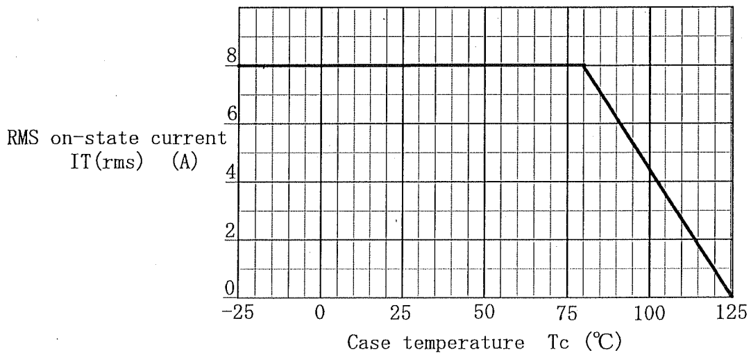
Fig.2 Tc-IT(rms) rating
