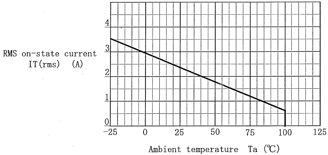
Fig.1 Ta-IT(rms) rating
