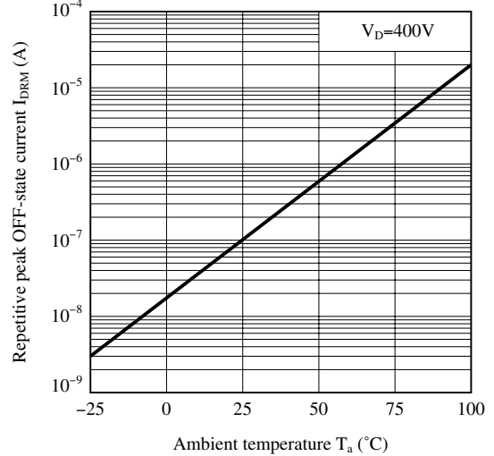
Fig.8-a Repetitive Peak OFF-state Current vs. Ambient Temperature (S116S01)
