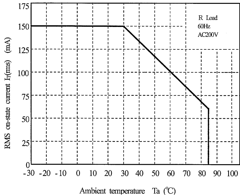
Fig.2 RMS on-state current I_T (rms) vs. Ambient temperature
