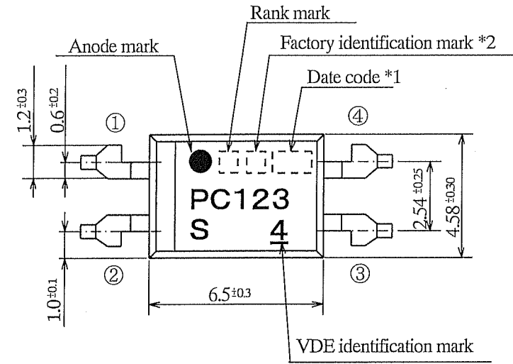
Pin-Number and internal connection diagram
