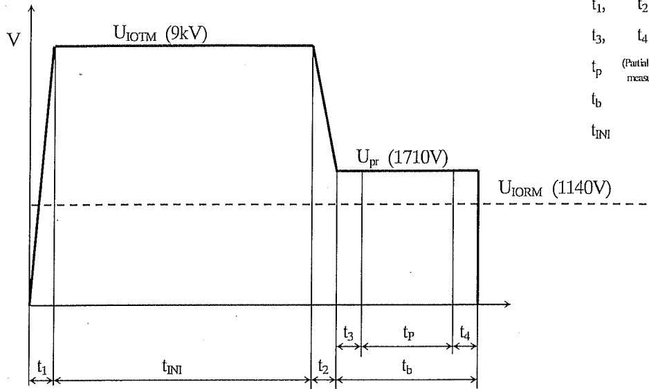
Method of Diagram 2: Non breakdown test (Apply to all device test)
